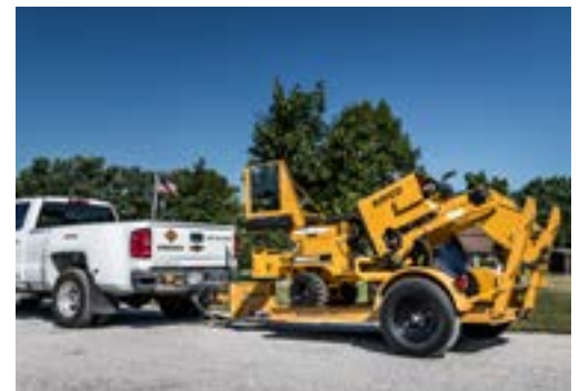
The TRG trailer is equipped with TorFlex suspension and electric brakes.
